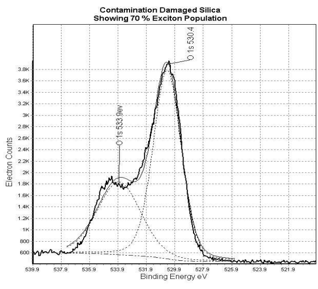
Figure 1 X-ray photoelectron spectrum of oxygen 1s electrons in a contamination related laser damaged optic, showing over 3.5 eV energy differentiation
